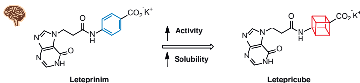
Figure 1. Modification and improvement of activity of Leteprinim drug.
