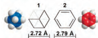
Figure 2. Comparison of 2- and 3-dimensional body views of cubane and benzene.
