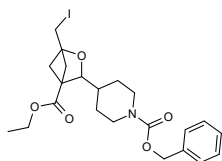
benzyl 4-[4-(ethoxycarbonyl)-1-(iodomethyl)-2-oxabicyclo[2.1.1]hexan-3-yl]piperidine-1-carboxylate
