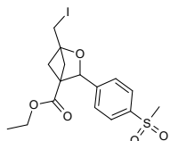
ethyl 1-(iodomethyl)-3-(4-methanesulfonylphenyl)-2-oxabicyclo[2.1.1]hexane-4-carboxylate
