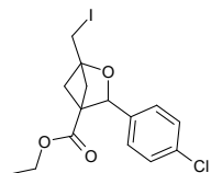
ethyl 3-(4-chlorophenyl)-1-(iodomethyl)-2-oxabicyclo[2.1.1]hexane-4-carboxylate
