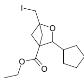
ethyl 3-cyclopentyl-1-(iodomethyl)-2-oxabicyclo[2.1.1]hexane-4-carboxylate
