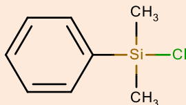
Chlorodimethylphenylsilane CAS: 768-33-2
