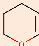
3,4-dihydro-2H-pyran CAS: 110-87-2
