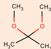
2,2-dimethoxypropane CAS: 77-76-9
