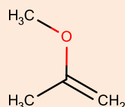
2-methoxyprop-1-ene CAS: 116-11-0
