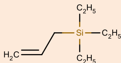
Allyltriethylsilane CAS:17898-21-4
