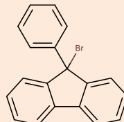
9-bromo-9-phenylfluorene CAS: 55135-66-5
