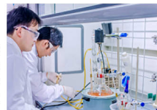
Cyclobutane Derivatives in Drug Discovery
