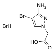
2-(3-amino-4-bromo-1H-pyrazol-1-yl)acetic acid hydrobromide
