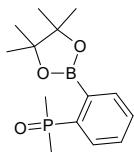
2-[2-(dimethylphosphoryl)phenyl]-4,4,5,5-tetramethyl-1,3-dioxaborolane
