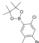
2-(4-bromo-2-chloro-5-methylphenyl)-4,4,5,5-tetramethyl-1,3-dioxaborolane
