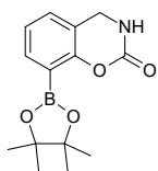
8-(tetramethyl-1,3,2-dioxaborolan-2-yl)-3,4-dihydro-2H-1,3-benzoxazin-2-one
