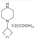
PBU12075-01 CAS: 1523571-19-8
