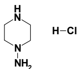
piperazin-1-amine hydrochloride
