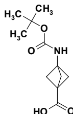
3-[[tert-butoxy]carbonyl]amino]bicyclo[1.1.1]pentane-1-carboxylic acid
