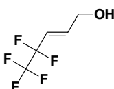
(E)-4,4,5,5,5-Pentafluoropent-2-en-1-ol
