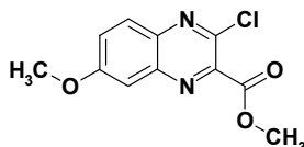
METHYL 3-CHLORO-7-METHOXYQUINOXALINE-2-CARBOXYLATE
