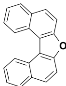
Dinaphtho[2,1-b:1',2'-d]furan
