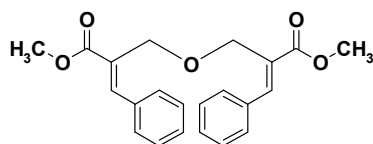
Dimethyl 2,2'-(oxybis(methylene))((2E,2'E)-bis(3-phenylacrylate))
