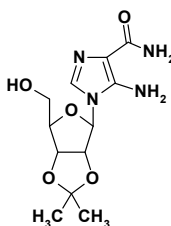
5-amino-1-[6-(hydroxymethyl)-2,2-dimethyl-tetrahydro-2H-furo[3,4-d][1,3]dioxol-4-yl]-1H-imidazole-4-carboxamide
