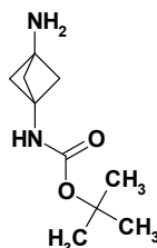
tert-butyl N-(3-aminobicyclo[1.1.1]pentan-1-yl)carbamate
