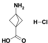
3-aminobicyclo[1.1.1]pentane-1-carboxylic acid hydrochloride
