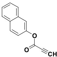
Naphthalen-2-yl propiolate
