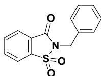
2-Benzylbenzo[d]isothiazol-3(2H)-one 1,1-dioxide
