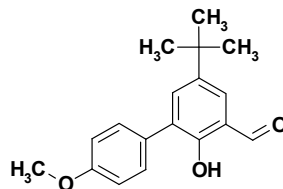
3-(4-methoxyphenyl)-5-tert-butylsalicylaldehyde
