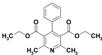
Diethyl 2,6-dimethyl-4-phenylpyridine-3,5-dicarboxylate
