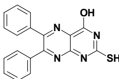
6,7-diphenyl-2-sulfanypteridin-4-ol
