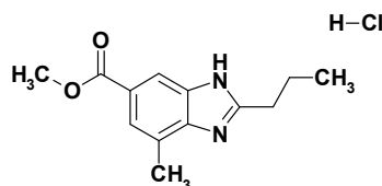
methyl 4-methyl-2-propyl-1H-1,3-benzodiazole-6-carboxylate hydrochloride
