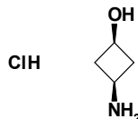
cis-3-Aminocyclobutanol hydrochloride
