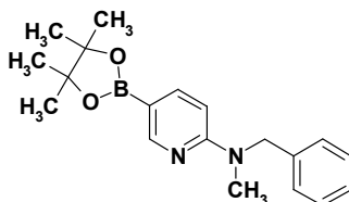
N-benzyl-N-methyl-5-(4,4,5,5-tetramethyl-1,3,2-dioxaborolan-2-yl)pyridin-2-amine
