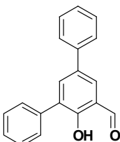
3,5-Diphenylsalicylaldehyde; 2-Hydroxy-3,5-diphenylbenzaldehyde
