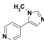
4-(1-methyl-1H-imidazol-5-yl)pyridine
