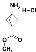
methyl 3-aminobicyclo[1.1.1]pentane-1-carboxylate hydrochloride
