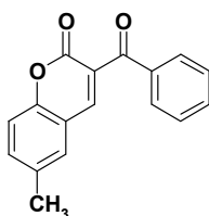
3-Benzoyl-6-methyl-2H-chromen-2-one
