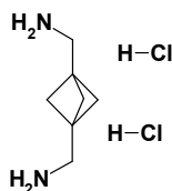
[3-(aminomethyl)bicyclo[1.1.1]pentan-1-yl]methanamine dihydrochloride
