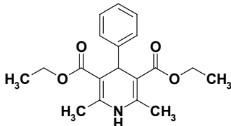
Diethyl 2,6-dimethyl-4-phenyl-1,4-dihydropyridine-3,5-dicarboxylate
