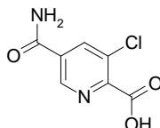
5-carbamoyl-3-chloropyridine-2-carboxylic acid
