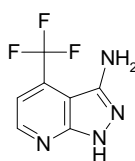
4-(trifluoromethyl)-1H-pyrazolo[3,4-b]pyridin-3-amine
