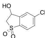
5-chloro-3-hydroxy-2,3-dihydro-1H-benzothiophene-1,1-dione
