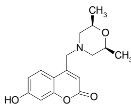
4-[(cis-2,6-dimethylmorpholin-4-yl)methyl]-7-hydroxy-2H-chromen-2-one
