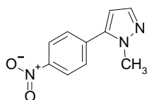
1-methyl-5-(4-nitrophenyl)-1H-pyrazole
